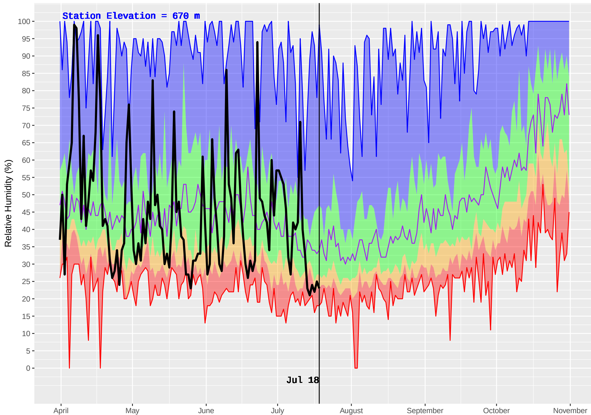
FINTRY (298) : Historical (1989–2016) and Current (2018) Daily Relative Humidity
