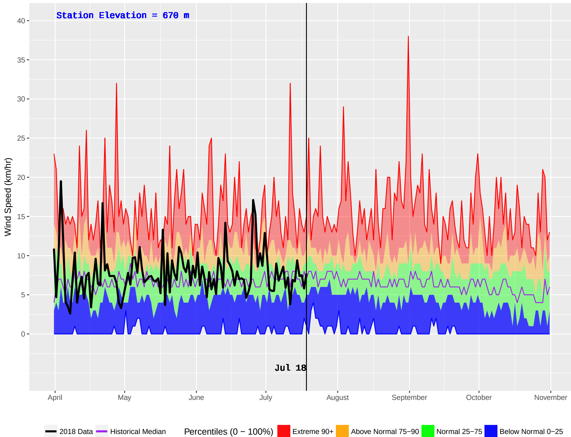
FINTRY (298) : Historical (1989–2016) and Current (2018) Daily Wind Speed
