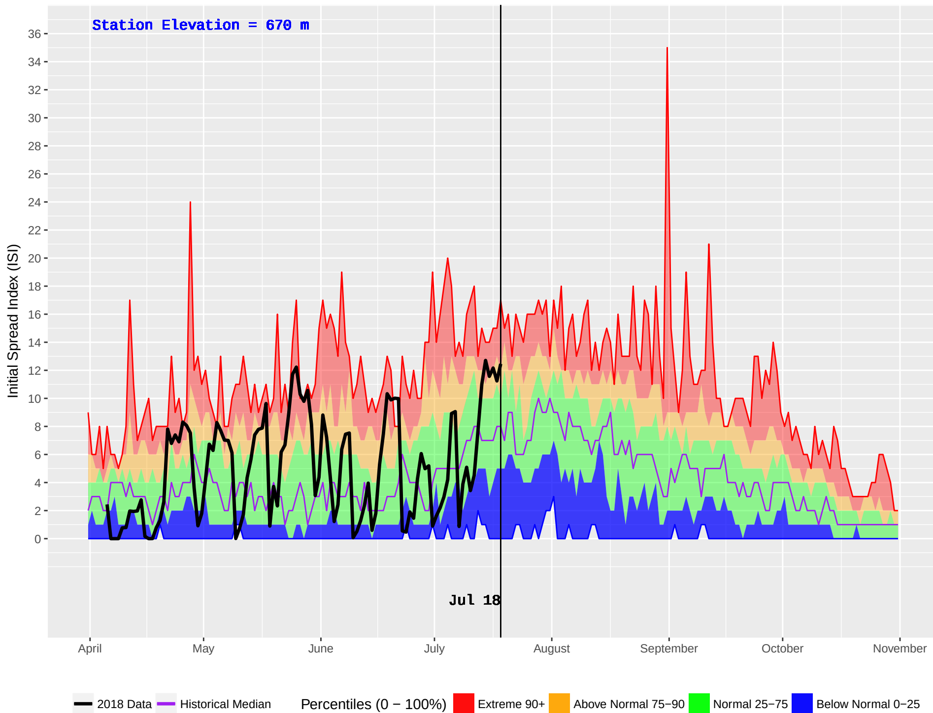
FINTRY (298) : Historical (1989–2016) and Current (2018) Daily Initial Spread Index (ISI)
