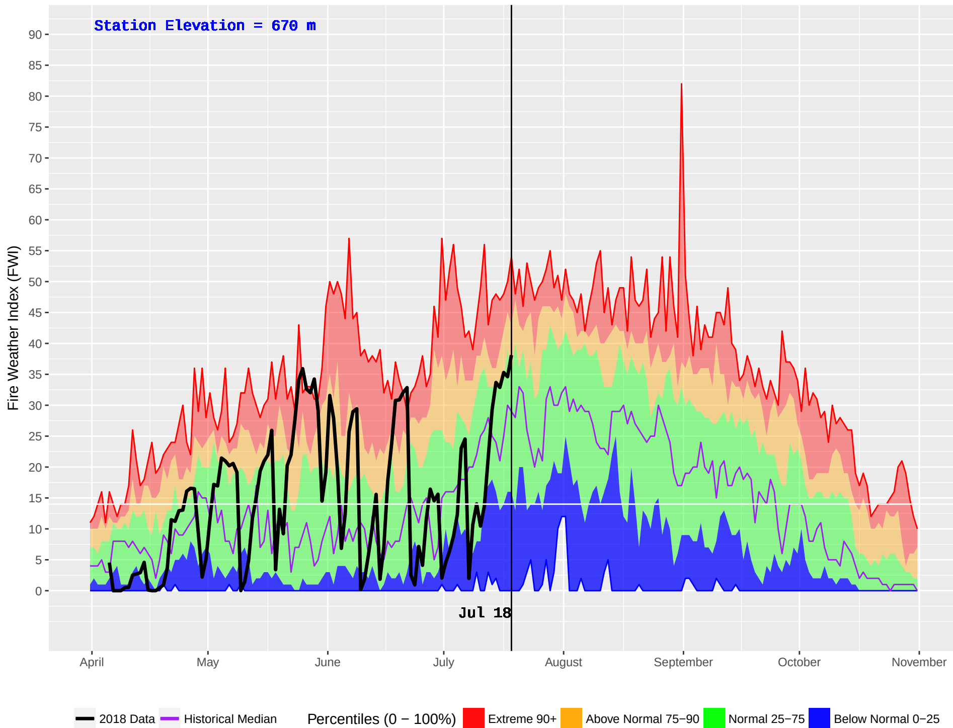
FINTRY (298) : Historical (1989–2016) and Current (2018) Daily Fire Weather Index (FWI)
