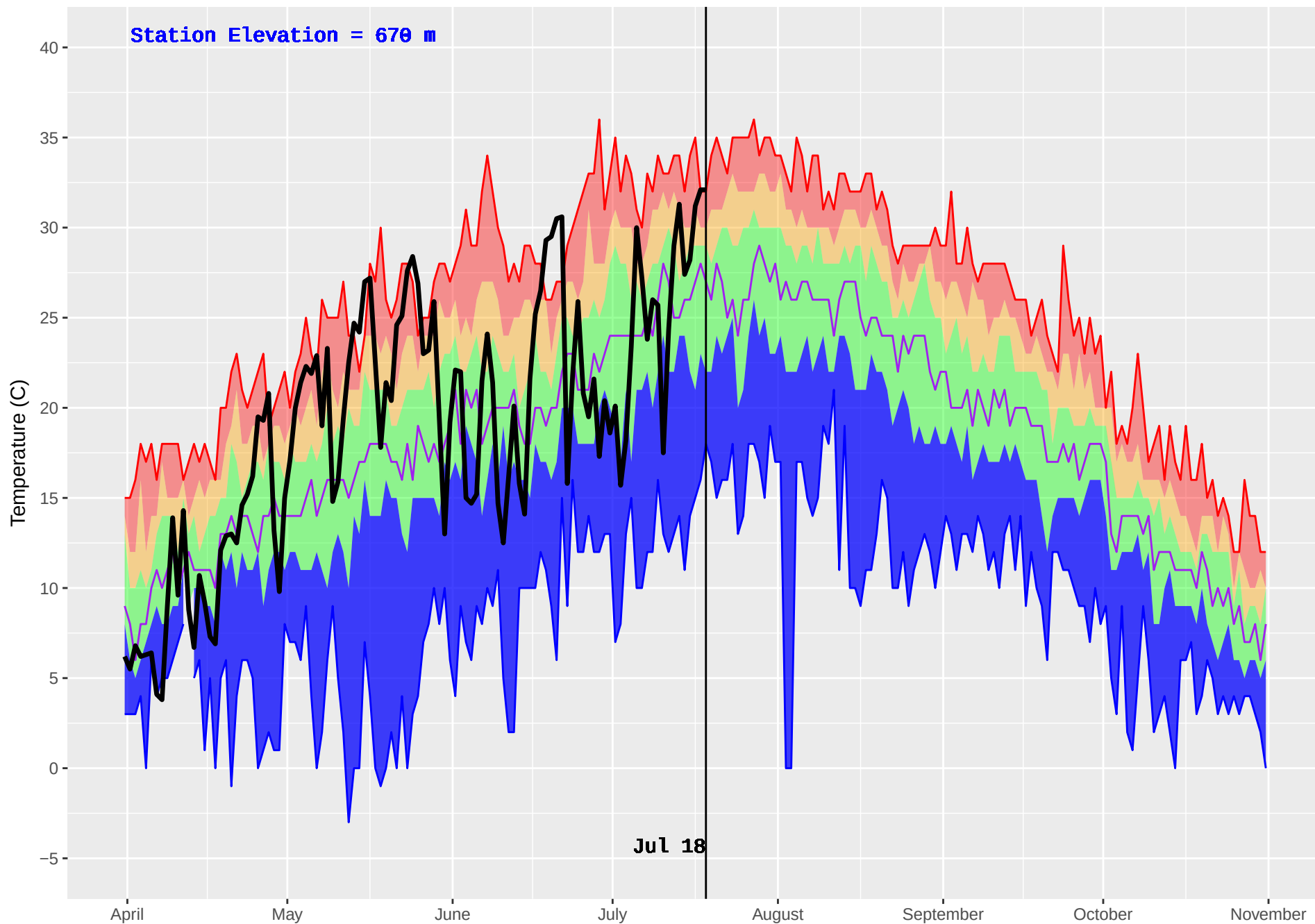
FINTRY (298) : Historical (1989–2016) and Current (2018) Daily Temperature
