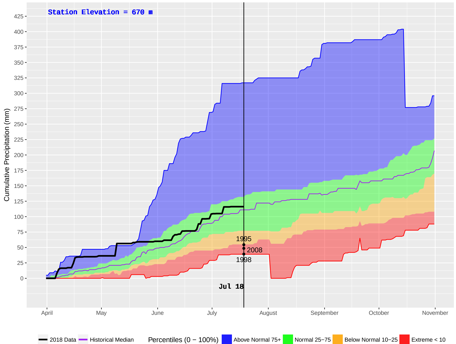
FINTRY (298) : Historical (1989–2016) and Current (2018) Daily Cumulative Precipitation
